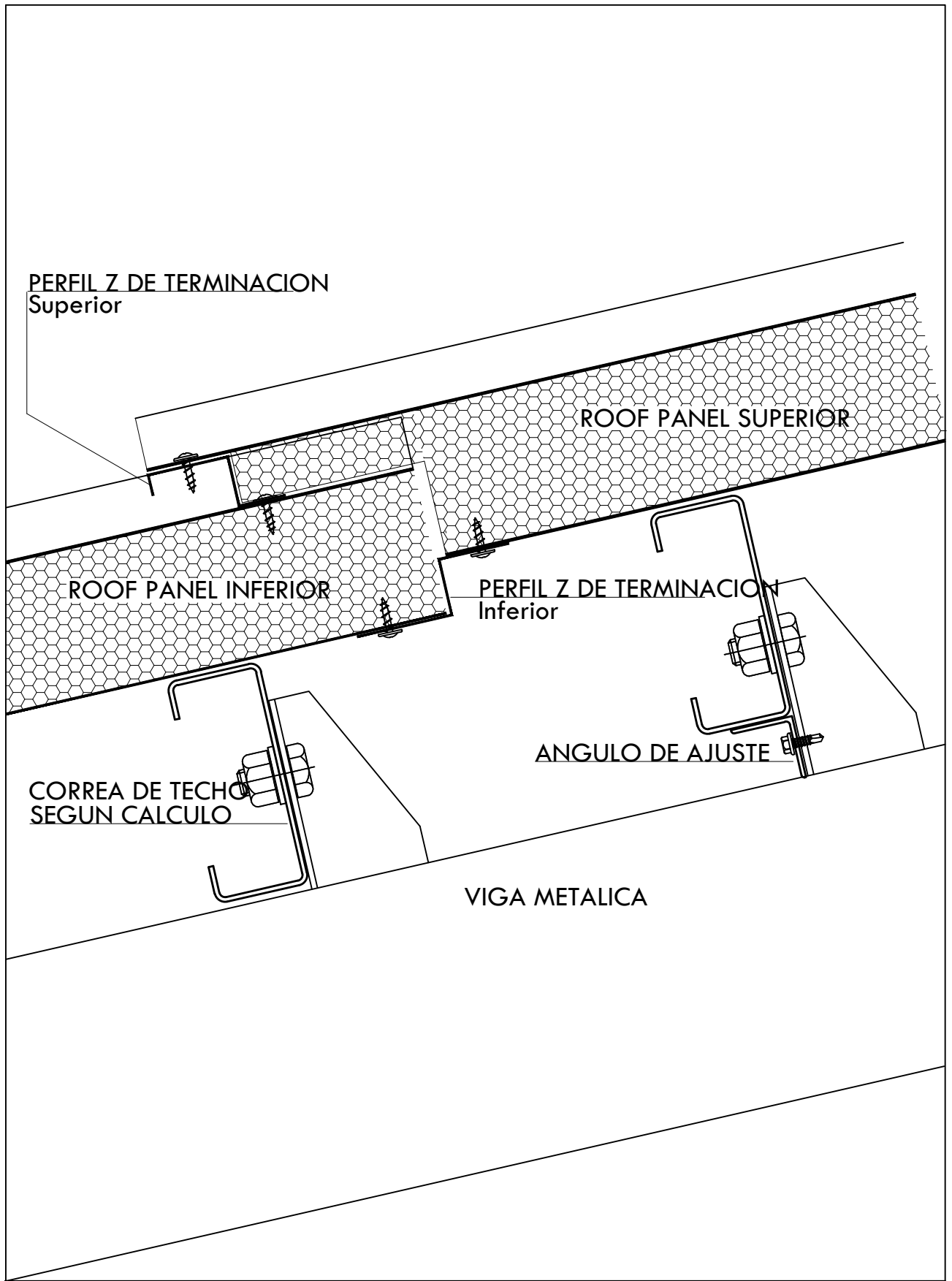
Solape de paneles Roof.
